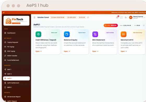
One hub: cash, balance, statement, eKYC
