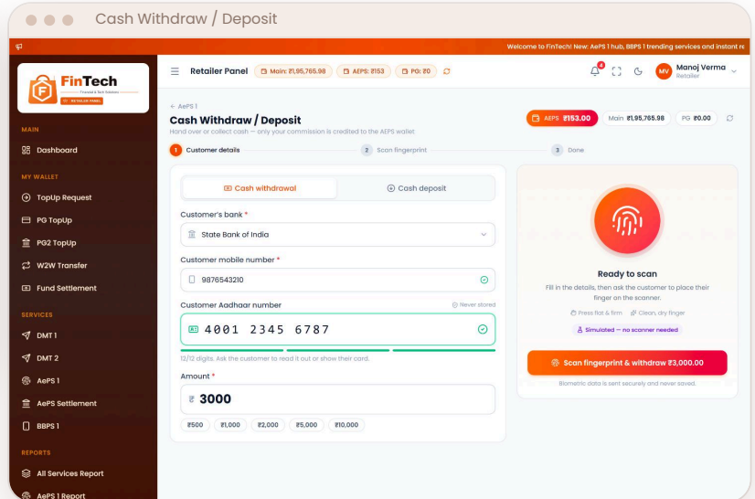
Aadhaar entry grouped 4-4-4 with validity tick, quick amounts and masked display
